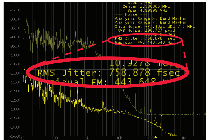
Figure 2. Femtosecond jitter.
